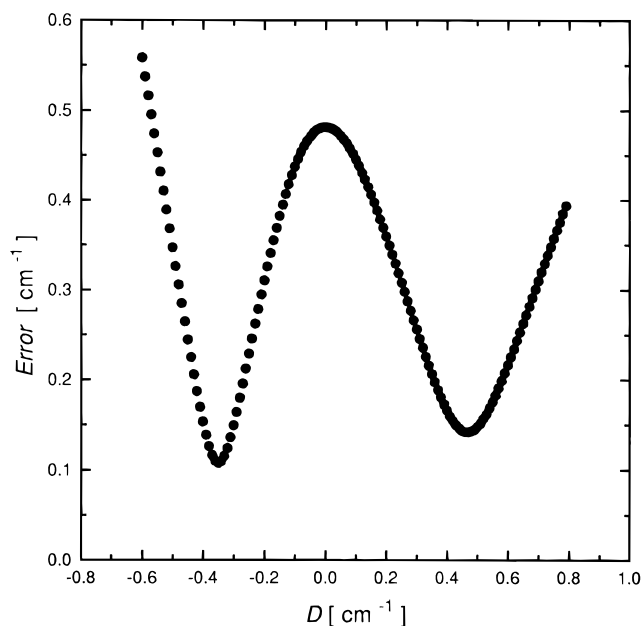
Figure 2. Plot of the error of fitting (least-squares) vs the axial zero-field splitting parameter ( D ) for the S = 9/2 ground state of [\text{Mn}_4\text{O}_3\text{Cl}(\text{O}_2\text{CMe})_3(\text{dbm})_3] ( 6 ). The data shown in Figure 1 were analyzed to give this plot of error vs D with the g value held constant at g = 1.995 .
